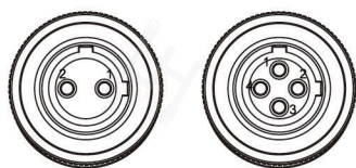
BCR Face View
